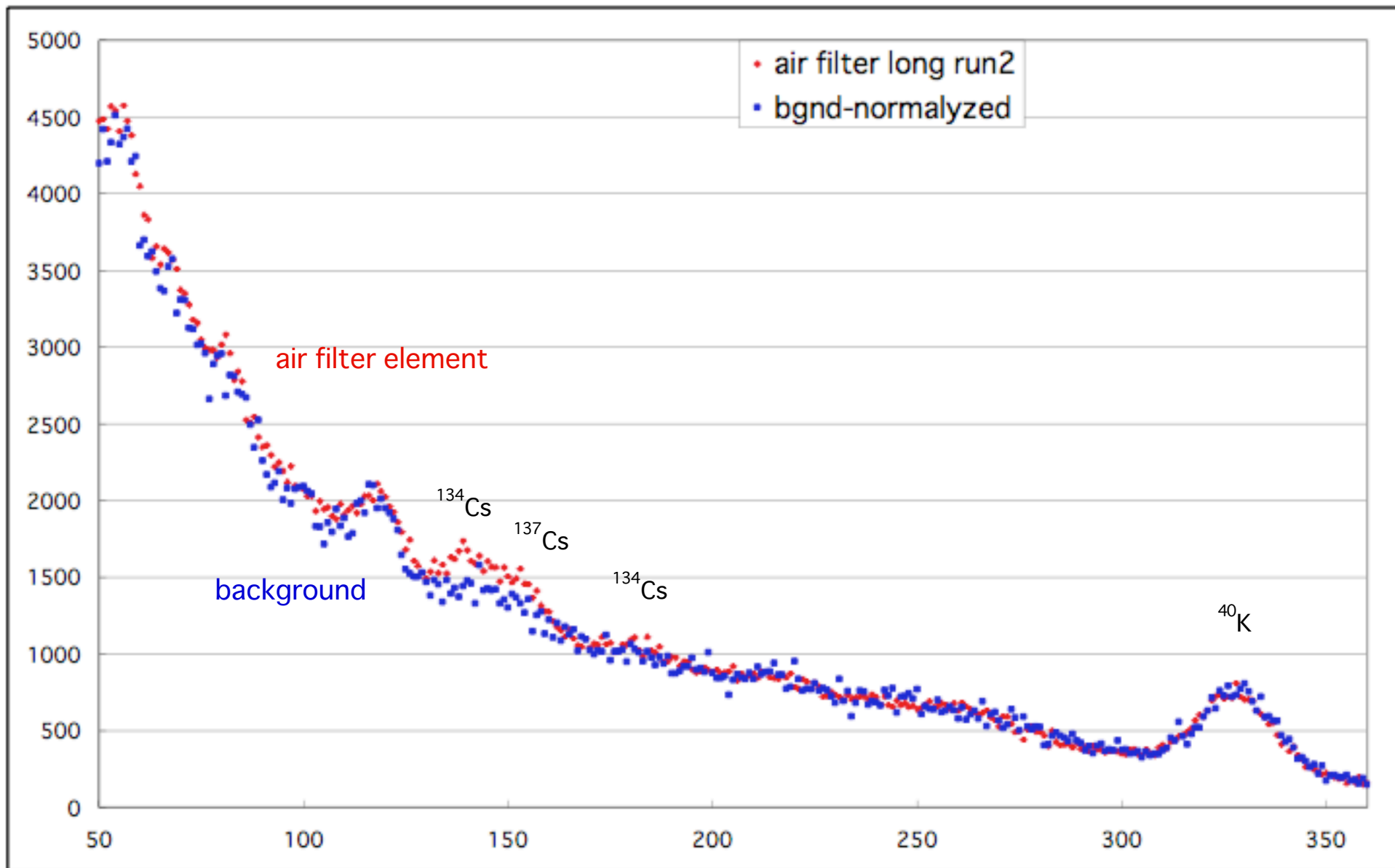
Gamma-ray spectrum from air filter exposed in Fukushima City. 21-22 Oct. 2011
